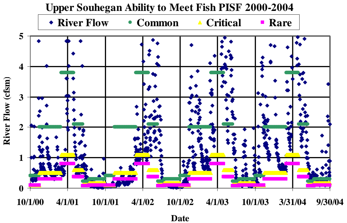
Figure 49b. Comparison of Fish PISF to Upper Souhegan River hydrograph for the last 5 years (magnified).
