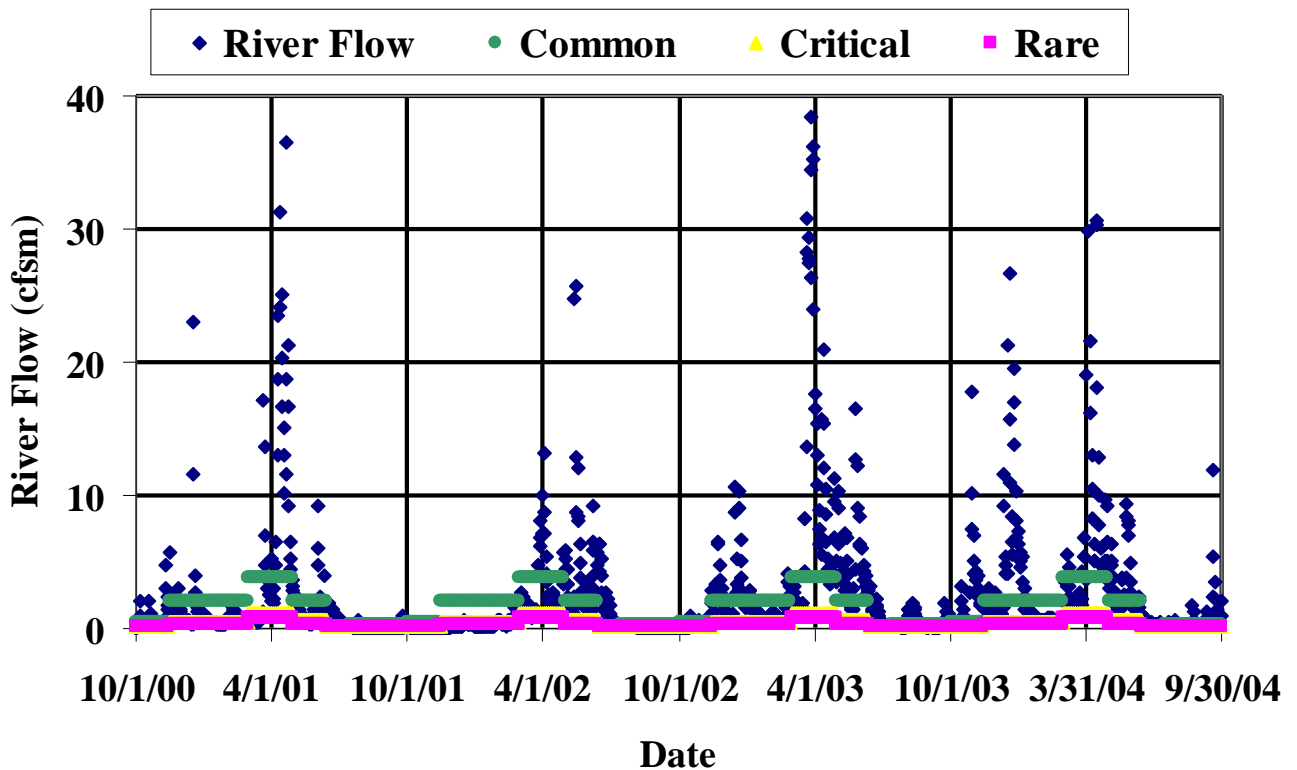
Upper Souhegan Ability to Meet Fish PISF 2000-2004
