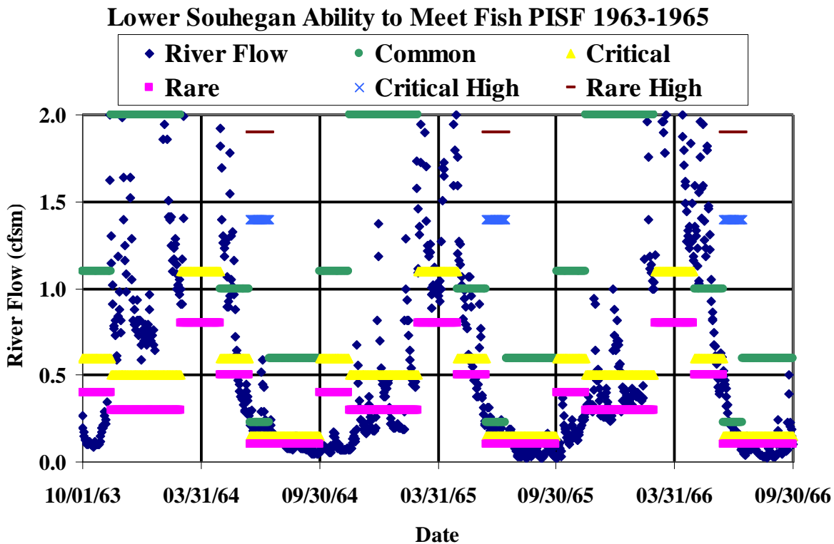
Figure 51. Comparison of Fish PISF to Lower Souhegan River hydrograph for the dry 3-year hydrograph.
