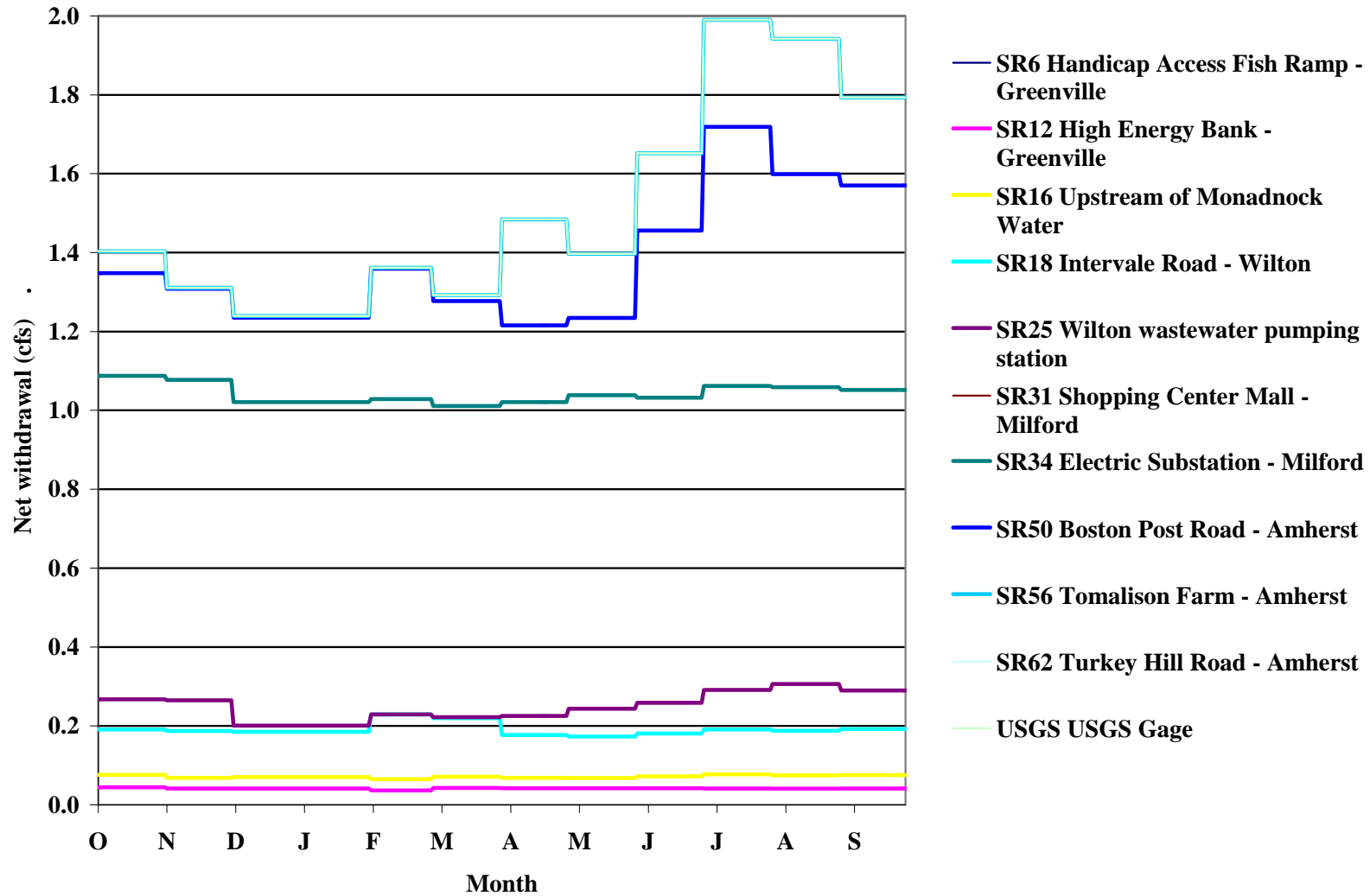
Figure 47. Monthly net withdrawal minus return flow (cfs). Values are to be added to the 5-year hydrograph for each reach.
