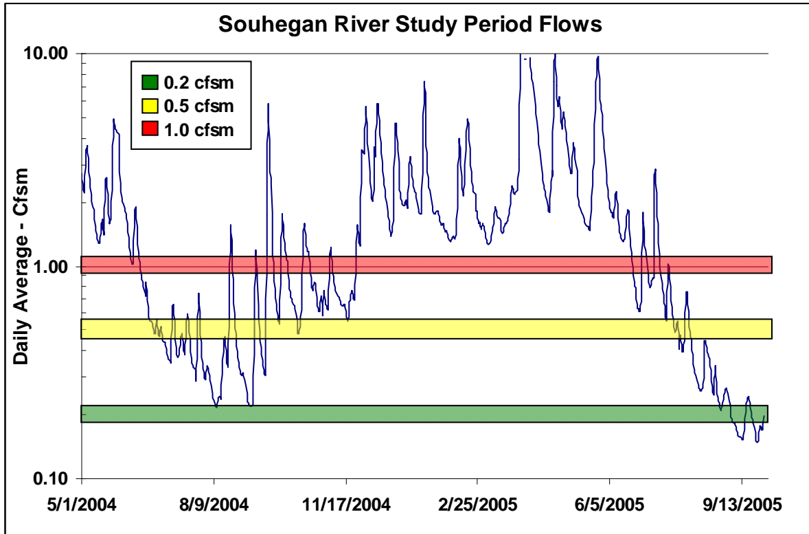
Figure 16. Hydrograph for the USGS stream gage at Wildcat Falls for the duration of the hydromorphological mapping period. The area shaded in green shows the river flow within 10% of 0.2 cfsm. The area shaded in yellow shows the river flows within 10% of 0.5 cfsm. The area shaded in red shows the river flows within 10% of 1.0 cfsm.
