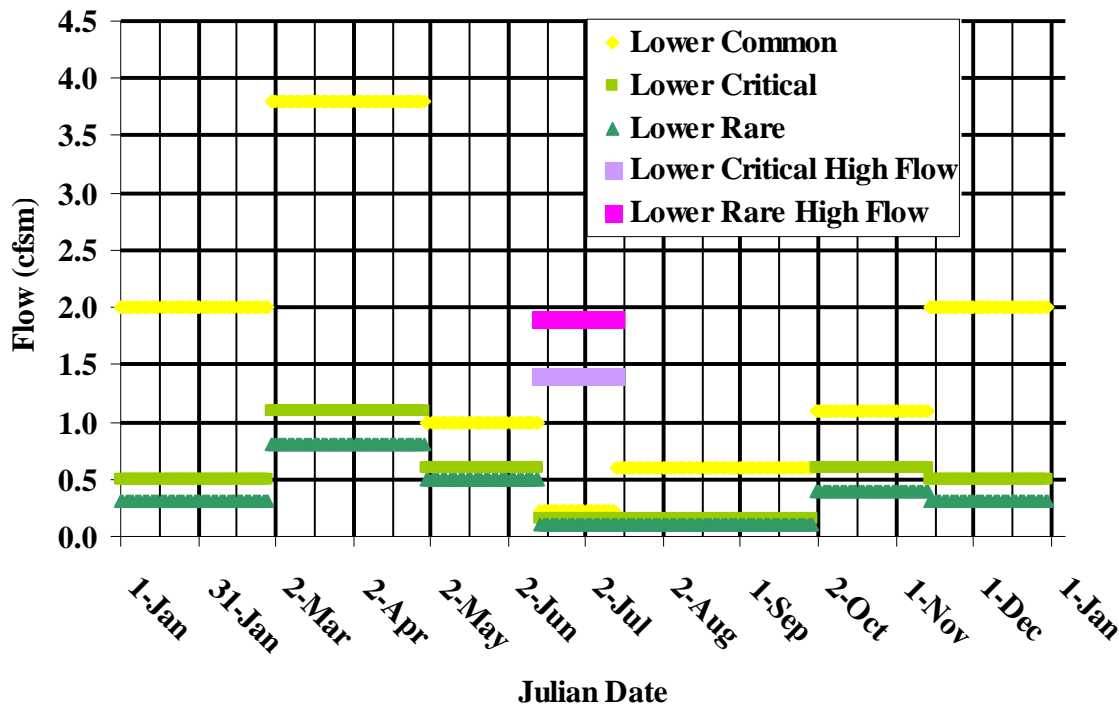
Figure 53. Synthesized PISF for the Lower Souhegan River.
