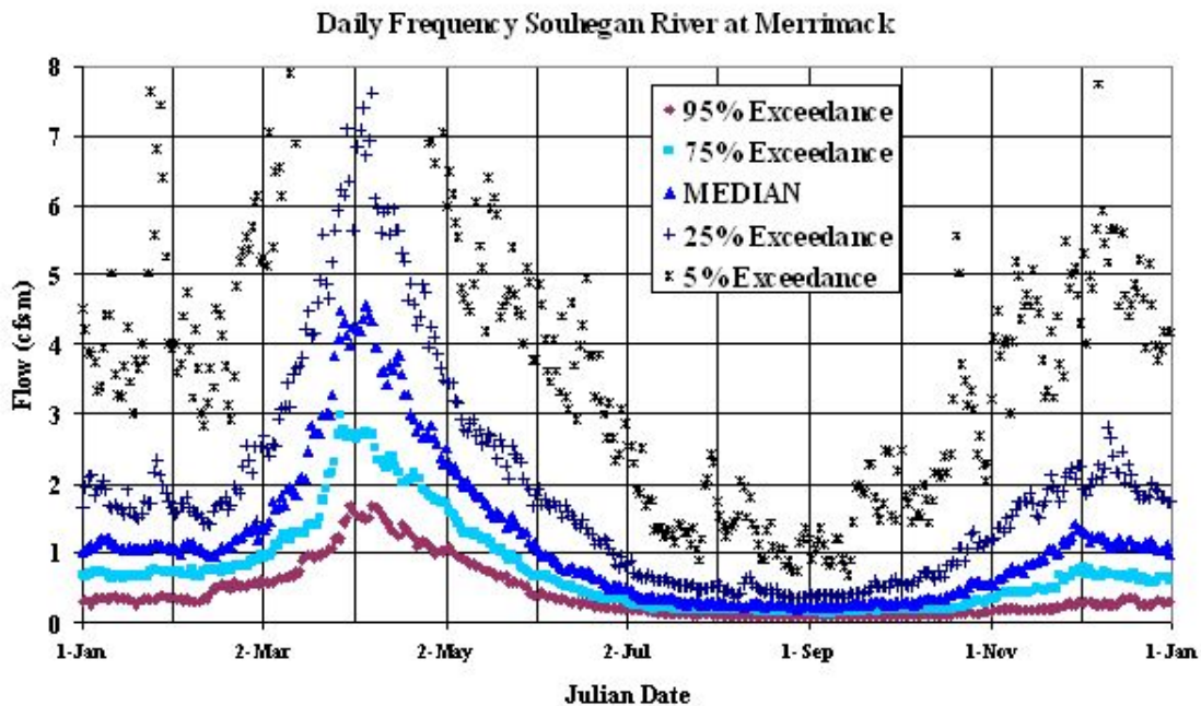
Figure 54. Daily flow frequency statistics for the Souhegan River (based on the USGS gage in Merrimack).
